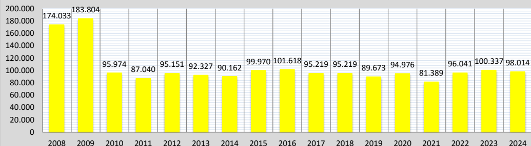
Strom [kWh]
